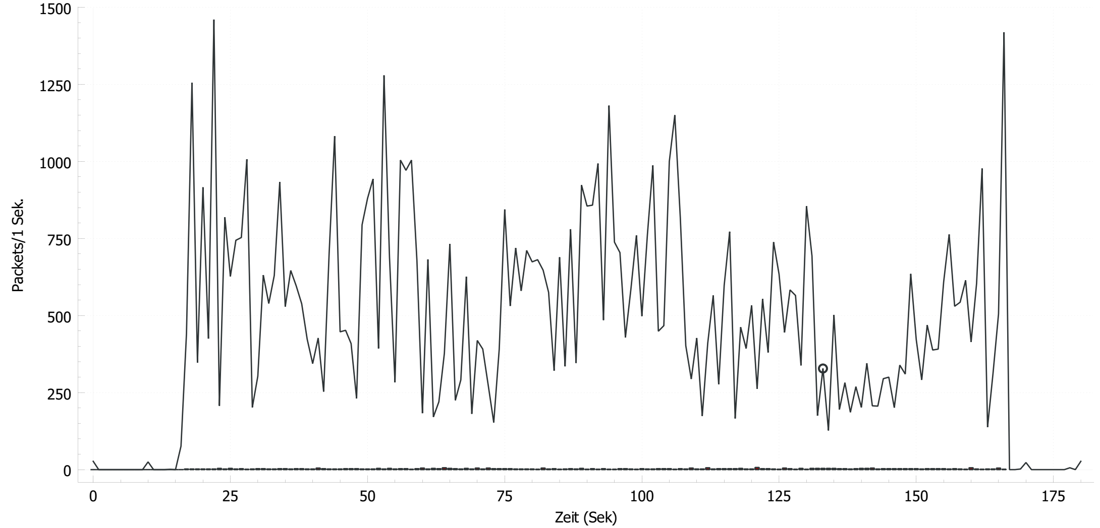
Wireshark I/O Graphen: copyGenZero.pcapng
